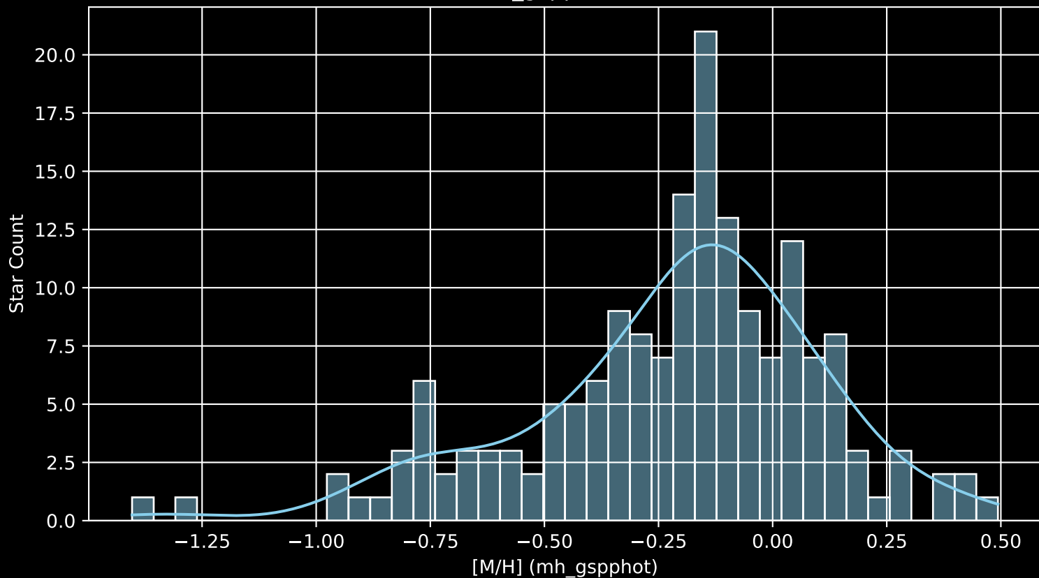
APOGEE DR17 Field: [226+31_MGA [M/H] (mh_gspphot) (n= 171)
