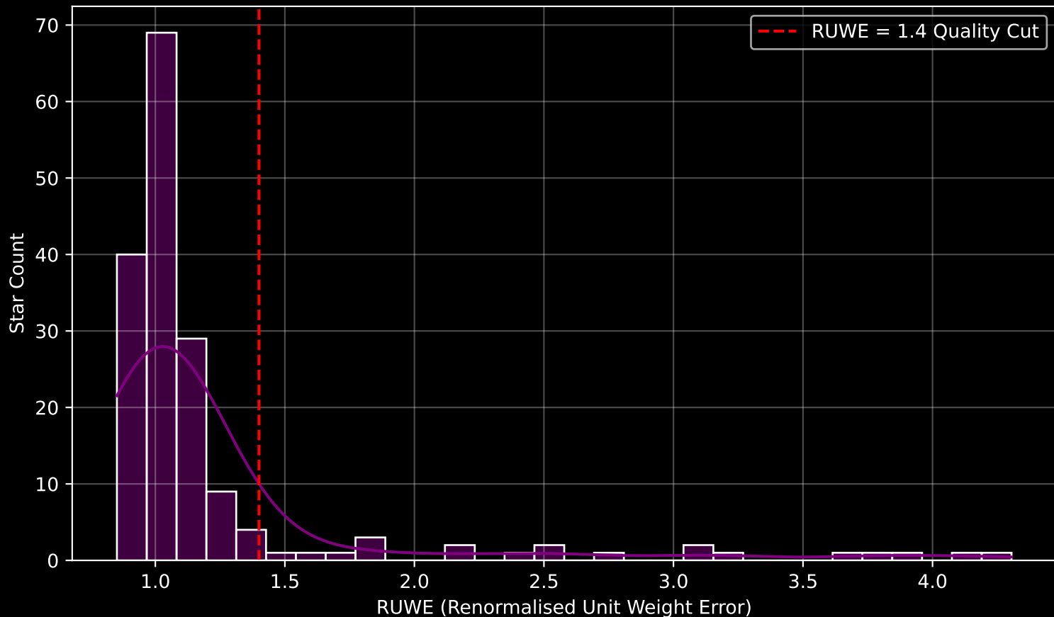
GAPOGEE DR17 Field [226+31_MGA] RUWE Distribution (n= 171)
