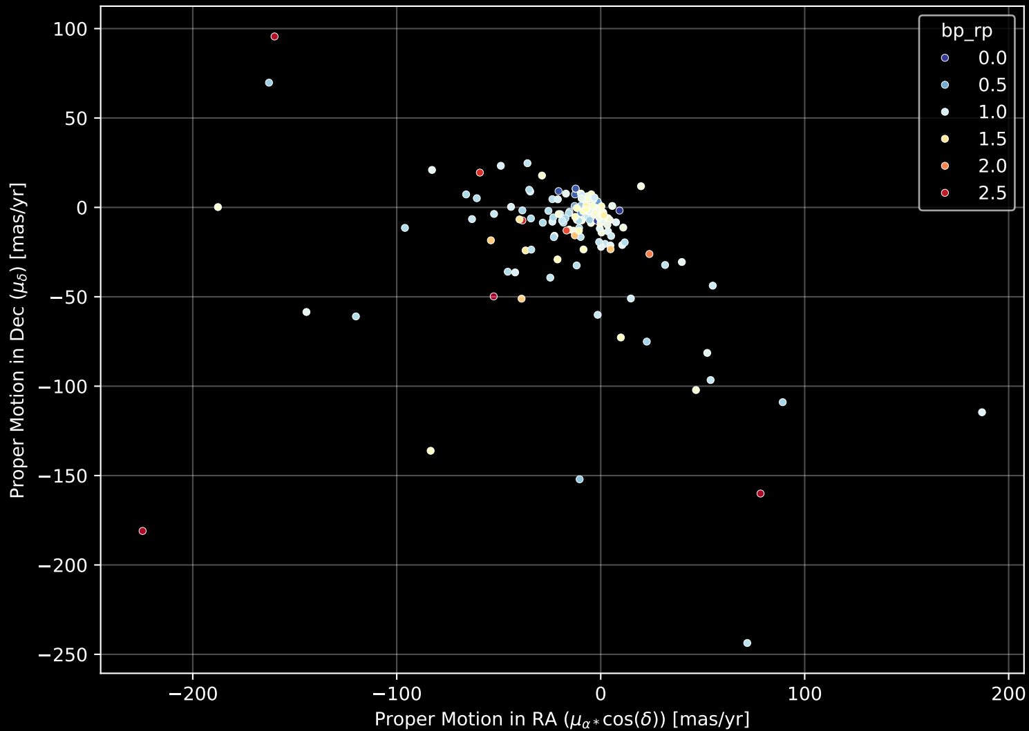
APOGEE DR17 Field: [226+31_MGA] Proper Motion Diagram (n= 172)
