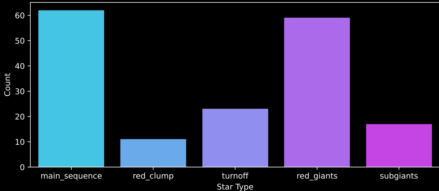
APOGEE DR17 Field: [226+31_MGA] Count plot of Star Type
