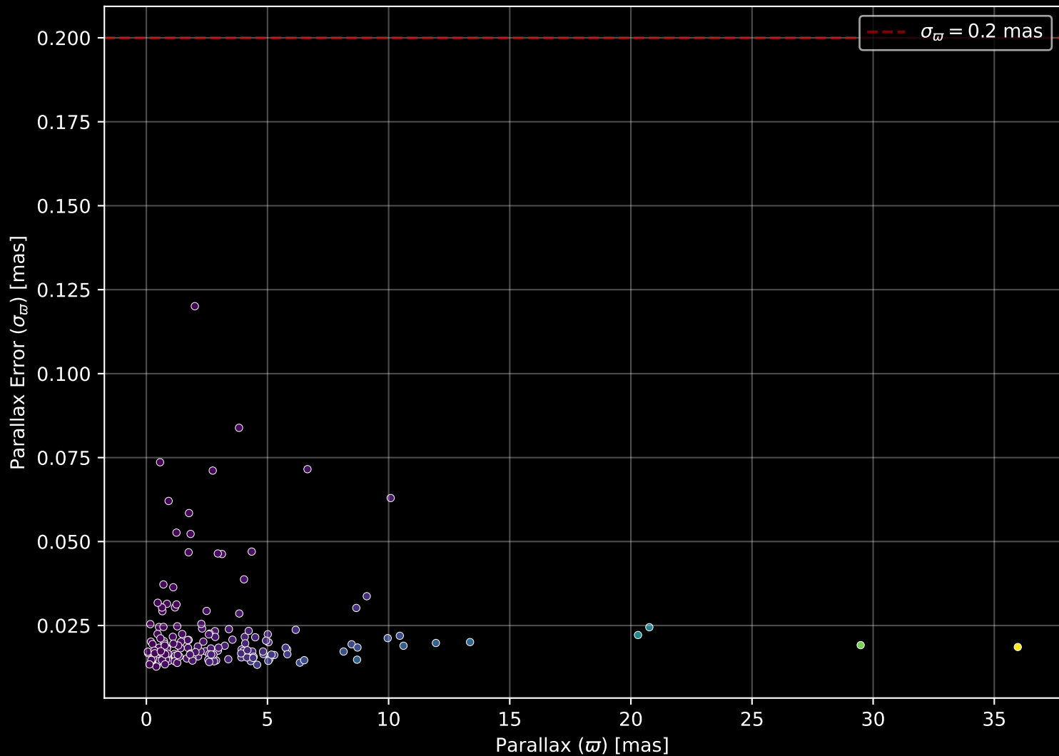
APOGEE DR17 Field: [226+31_MGA] Parallax Quality (n= 172)
