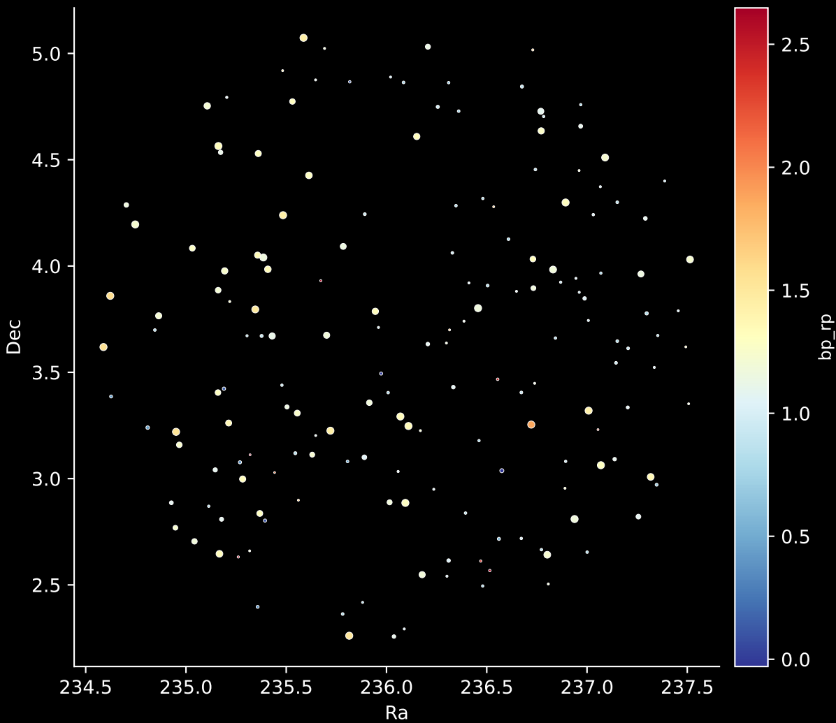
APOGEE DR17 Field: [226+31_MGA] Stars: 172
