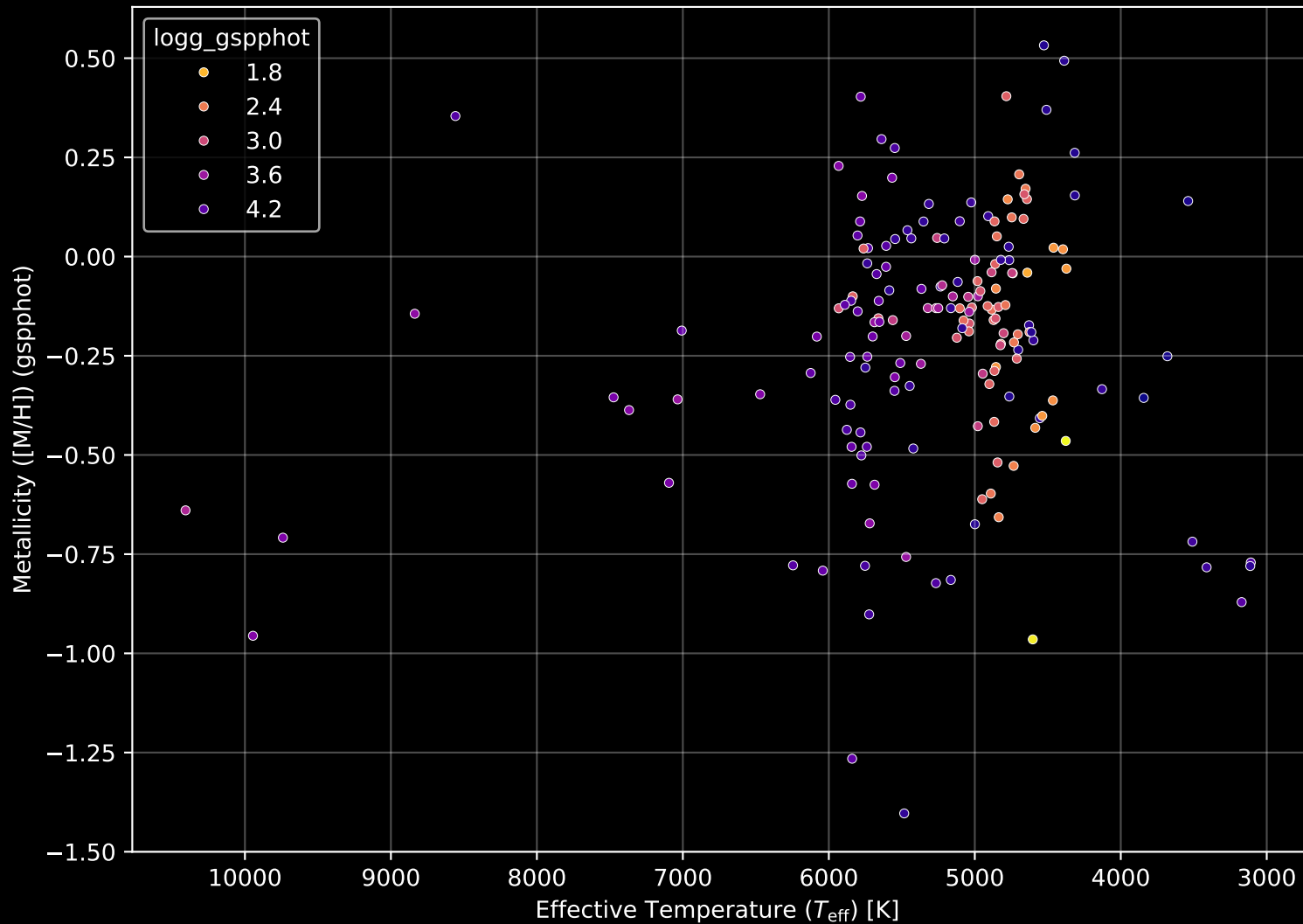
APOGEE DR17 Field: [226+31_MGA] Stellar Population Parameters (n= 172)
